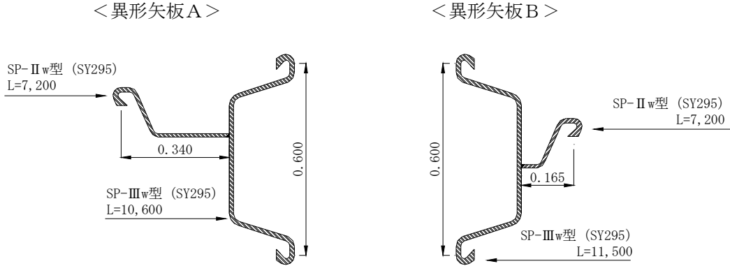
[異形矢板計算例]
