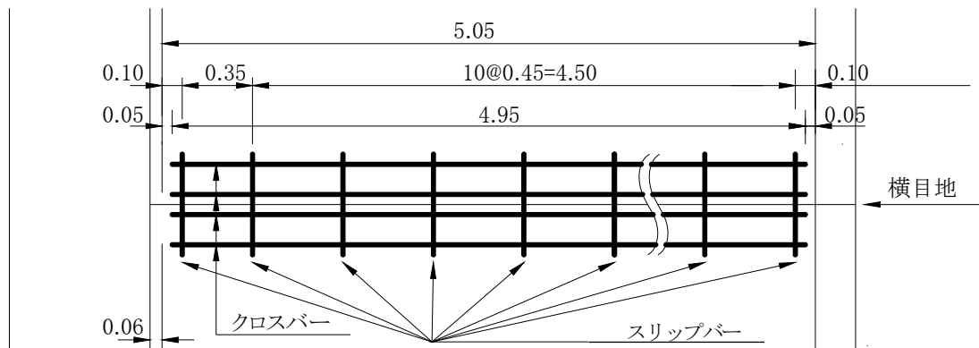
[断面図]
