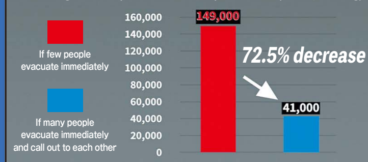
According to the Japan Trench Earthquake model (winter, evening)
