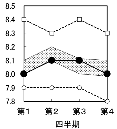
図3-3 pH
