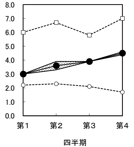
図5-7 強熱減量(%)
