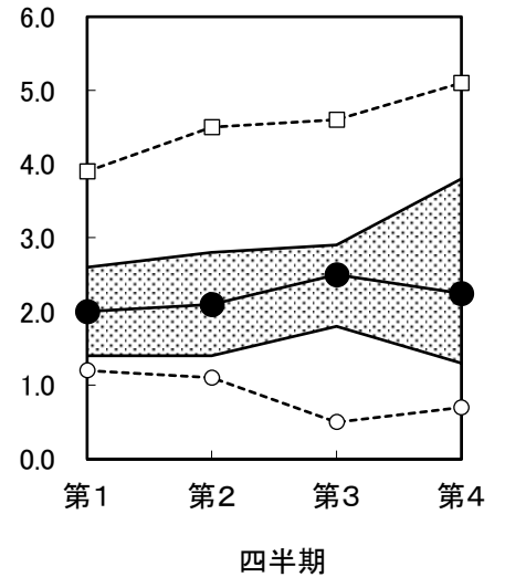
図5-3 強熱減量(%)
