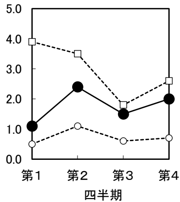
図4-5 COD(mg/L)
